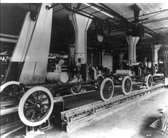
Linia de asamblare la Fabrica Ford Motor Company din Highland Park, 1913
